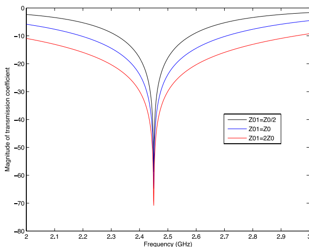
Figure 2. Response of the stub filter at 2.45GHz for different Z_{01}/Z_0 ratios.
