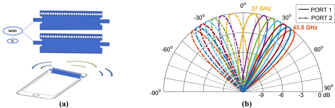
Figure 1. a) LWA design b) Frequency-scanned radiation using the channels available in the 36-40 GHz band
