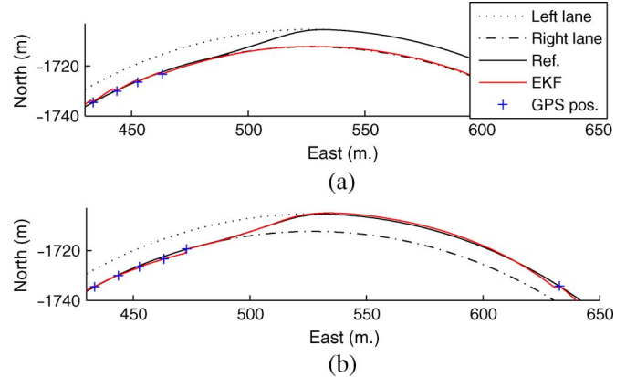
Fig. 4. Stretch of the N30 circuit with (a) the KL model and (b) the CL model. Right lane (dash-dotted black line), left lane (dotted black line), Ground truth (solid black), EKF model trajectory (solid red), and GPS points (blue +). A GPS mask of 15 s is assumed.
