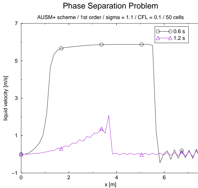
FIGURE 5.42. Liquid velocity
