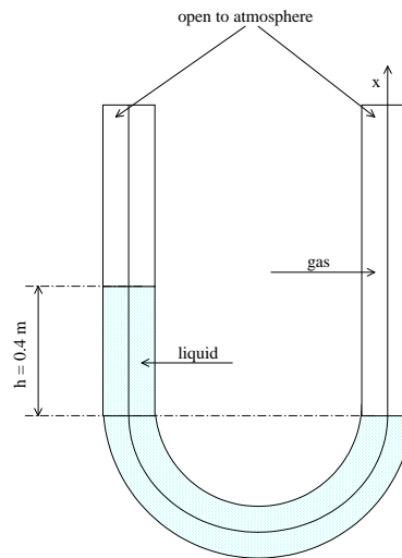
FIGURE B.5. Scheme of the oscillating water column in a U-tube manometer.
