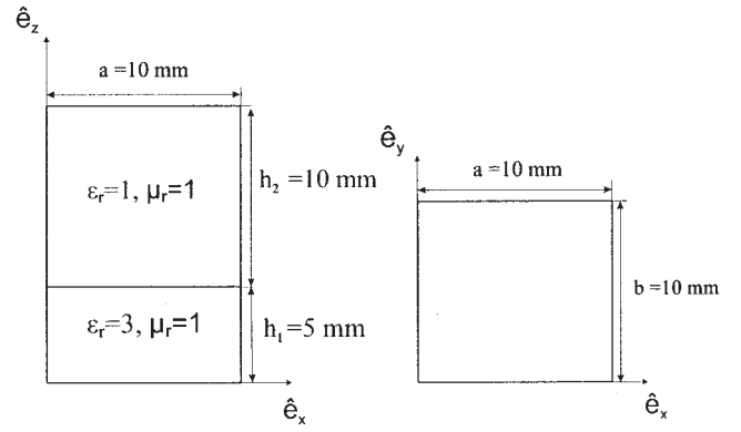
Figure 2 Shielded microstrip multilayered structure
