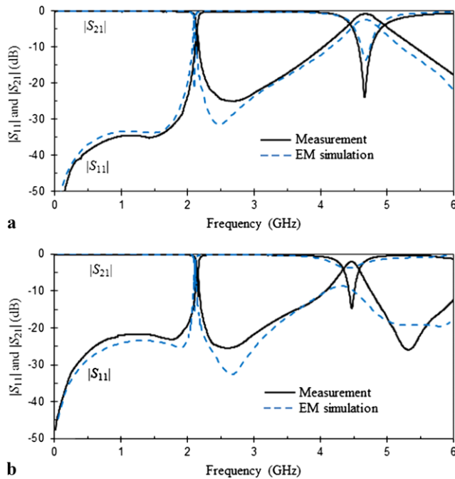
Fig. 6 EM simulation ( dashed lines ) and measured ( solid lines ) results for the microstrip line loaded with an OISRR: (a) D_1 \times D_2 = 9 \times 9 \text{ mm}^2 and (b) D_1 \times D_2 = 14 \times 9 \text{ mm}^2 . OISRR data: r = 2.2 \text{ mm} , c = 0.3 \text{ mm} and s = 0.25 \text{ mm}
