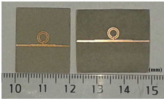
Fig. 5 Photographs of the fabricated microstrip notch filters
