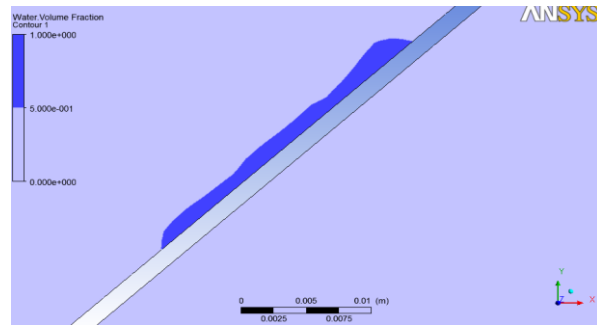
Figure 17. Images of experimental and numerical water film over the plate.
