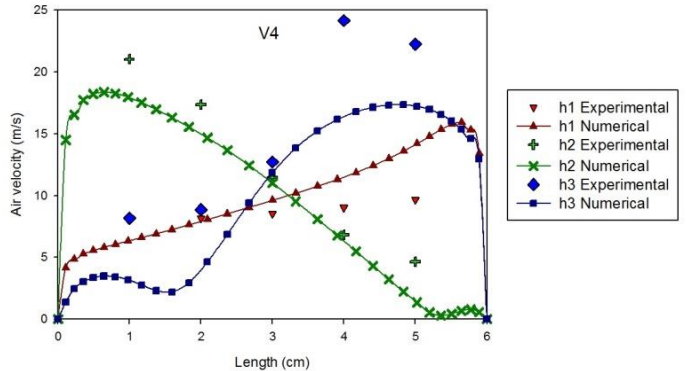
Figure 15. Air velocities for V4 at the air entrance section.
