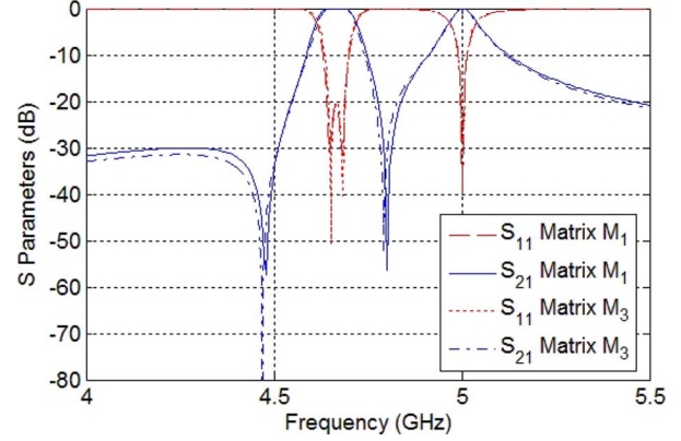
Fig. 4. Response of the coupling matrix M_3 versus the original prototype function (matrix M_1 ).
