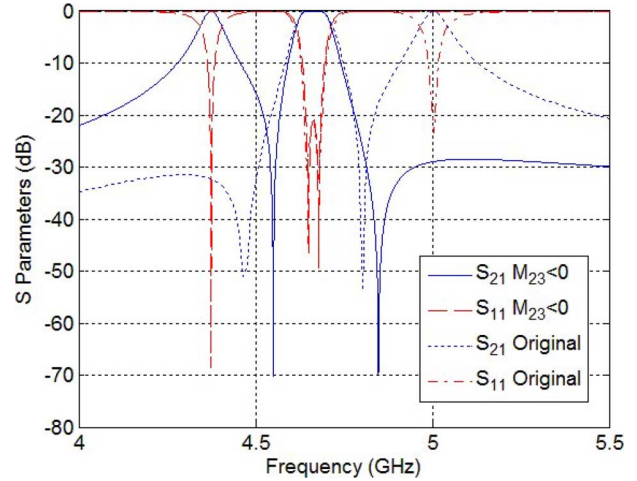
Fig. 9. Ideal model ( M_4 , but with M_{23} < 0 ) versus full wave simulated results of the original response (with b = 34 mm).
