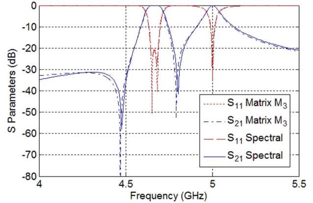
Fig. 6. Ideal model ( M_3 ) versus full wave simulated results of the designed hybrid structure.
