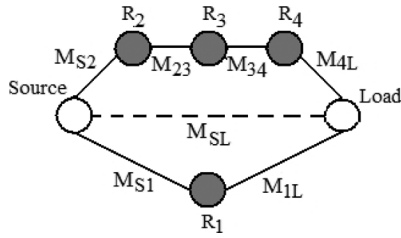
Fig. 10. Coupling scheme of a fourth-order fully canonical filter. Again, M_{SL} represents the direct coupling from source to load.
