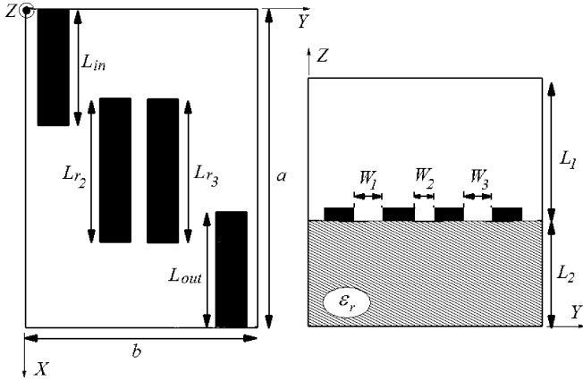
Fig. 1. Hybrid waveguide-microstrip structure for a third-order dual-bandpass filter following the coupling topology shown in Fig. 2. The width of the microstrip resonators, and of the input/output ports in the examples of this paper is 2 mm.
